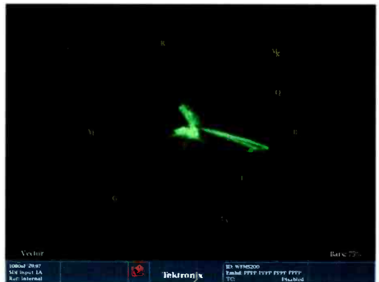
Figure 3. A vectorscope is an XY plot of color (hue) as an angular component of a polar display, much like some familiar color wheels used in color graphics.
